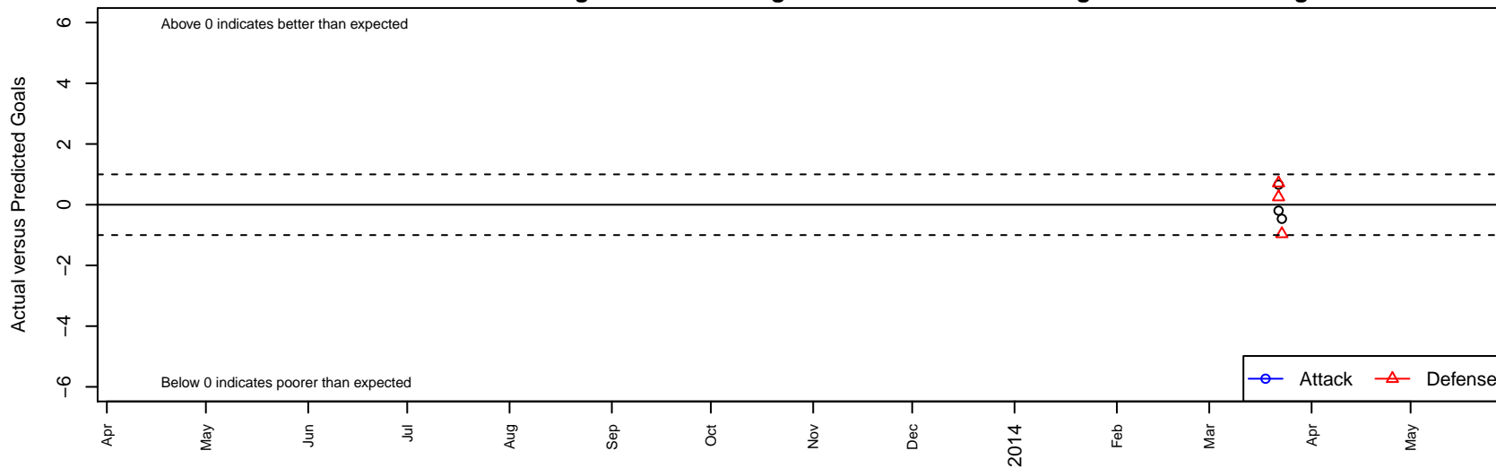
San Juan SC 96 Lightning Blue B95 Dots are actual minus expected GF (blue circles) and GA (red triangles). Blue line is smoothed change in attack strength. Red is smoothed change in defense strength.
